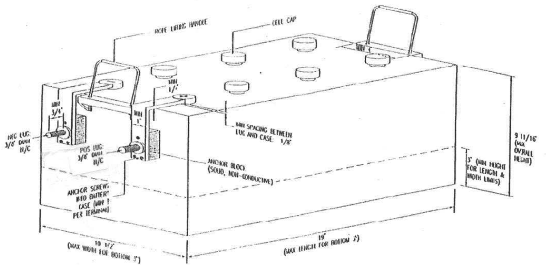
BUS BATTERY WITH DROP TERMINALS – Dimensional Specifications –
